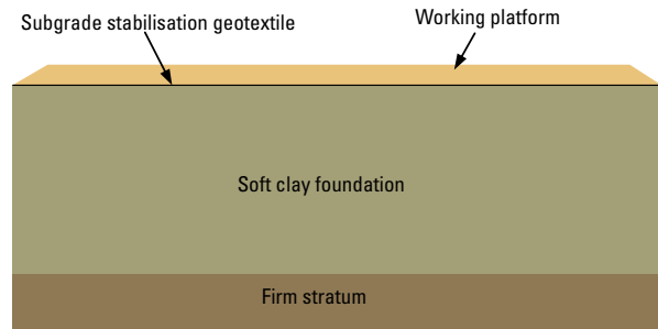
a) Construction of working platform on top of soft clay foundation
